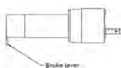
Rotate approx. 30 degrees counter-clockwise to release motor brake
