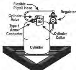
Single Cylinder
